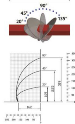
Cutting diagram (tolerance +/- 3mm)
